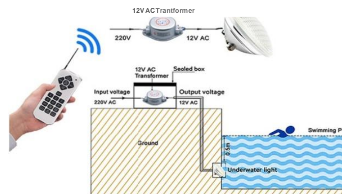
PAR56 REMOTE CONTROL CONNECTED DIAGRAM
